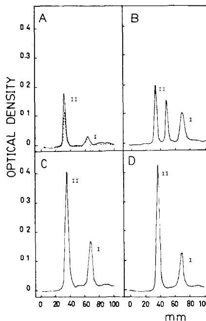
Fig.3. Electrophoretic analysis of the CNBr fragments of 32 P-labeled glycogen synthase. Samples of the immunoprecipitates were cleaved with CNBr before being subjected to electrophoresis in 15% acrylamide gels. Autoradiograms were obtained and then scanned. (A,C,D) Immunoprecipitates of 32 P-labeled glycogen synthase obtained from control (A), epinephrine (C) and vasopressin (D) treated hepatocytes. (B) The pattern of CNBr cleavage products of partially proteolyzed glycogen synthase. The dotted lines in (A) correspond to CNBr fragments of purified glycogen synthase phosphorylated in vitro with the catalytic subunit of cAMP-dependent protein kinase.
